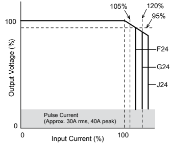
Overcurrent Protection Characteristics PS6R-□24
